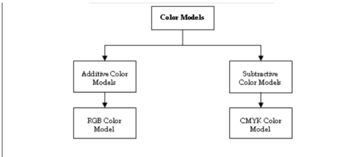
Fig 5.12: Color Models
