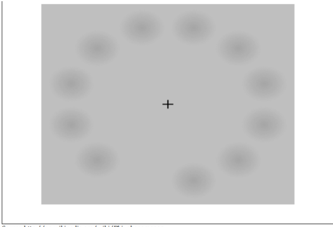
Fig 5.15: Phi Phenomenon
