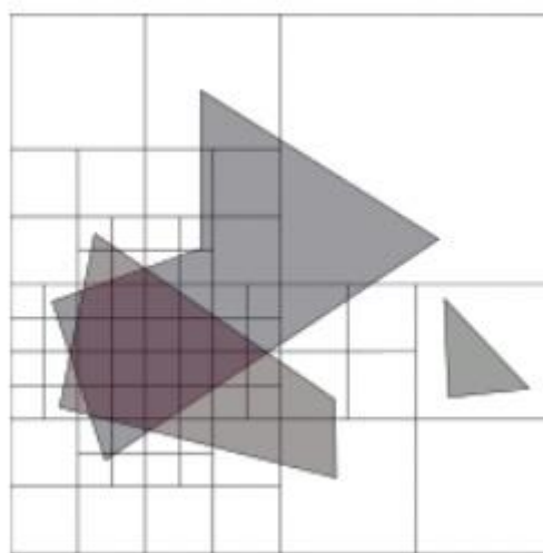
Fig.5.5. Warnock algorithm
