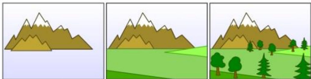
Fig 5.4: Painter's Algorithm
