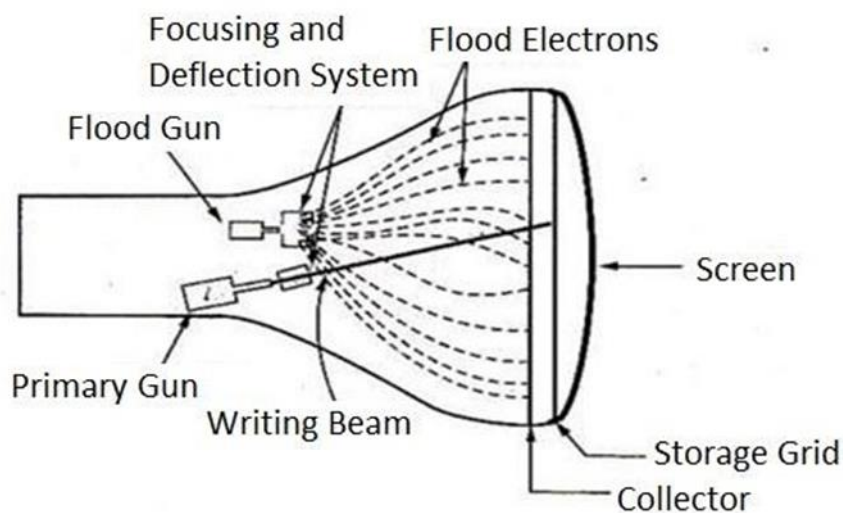
Fig 1.15: Direct-view storage tube
