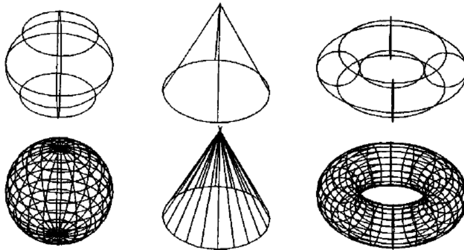
Fig. 2.21 Effect of Mesh Size on Object Visualization
