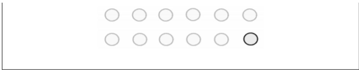
Fig 5.16: Beta Phenomenon
